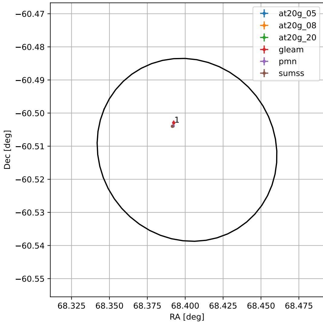
4FGL J0433.6-6030
