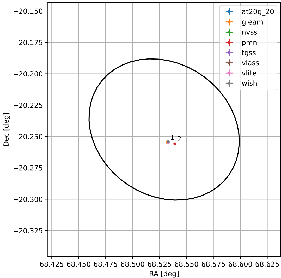
4FGL J0434.1-2014
