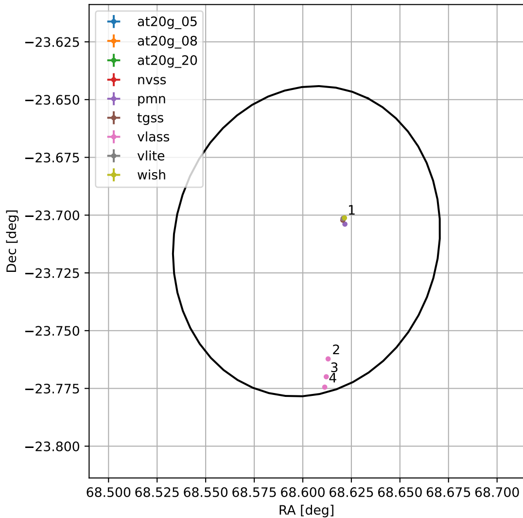
4FGL J0434.4-2342
