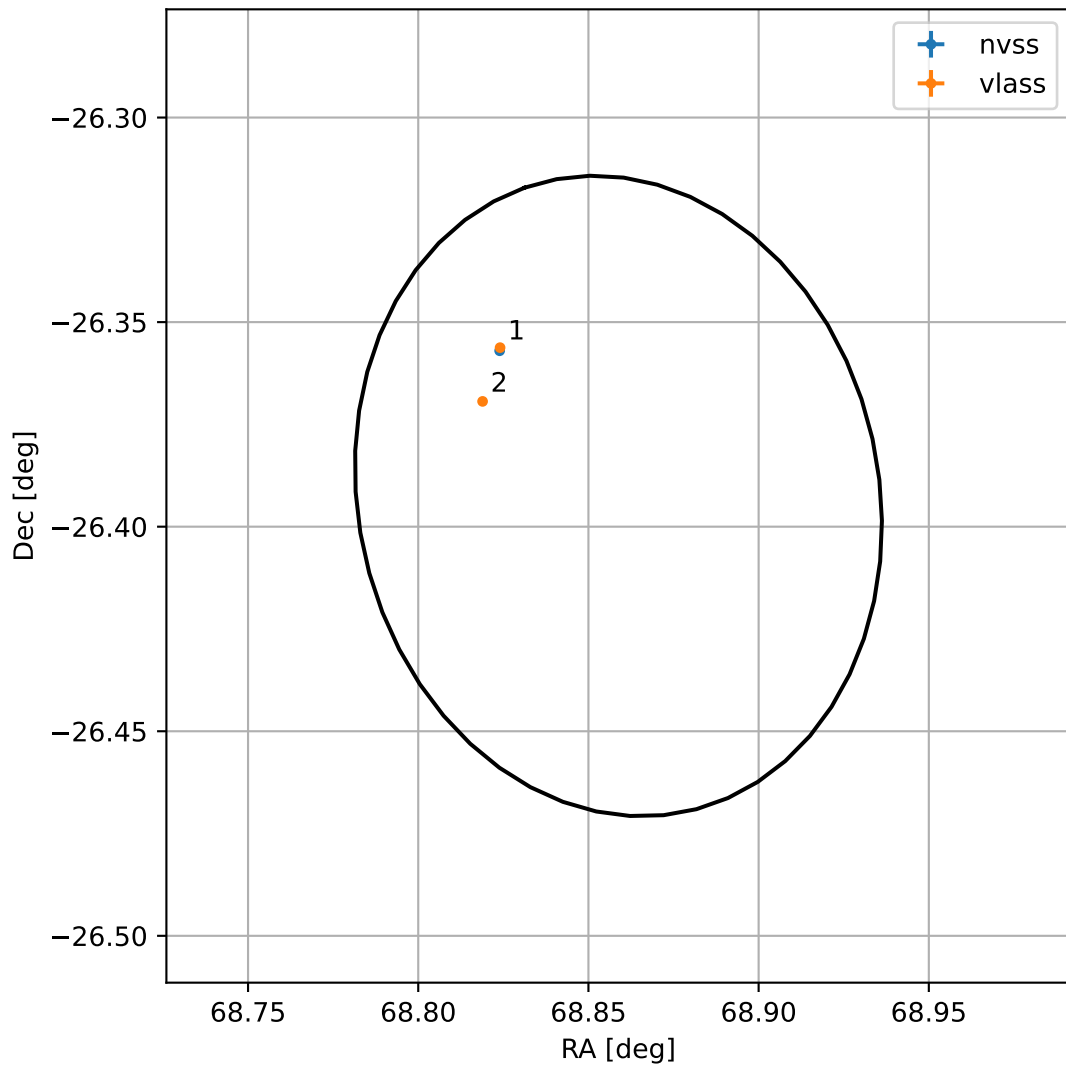
4FGL J0435.4-2623
