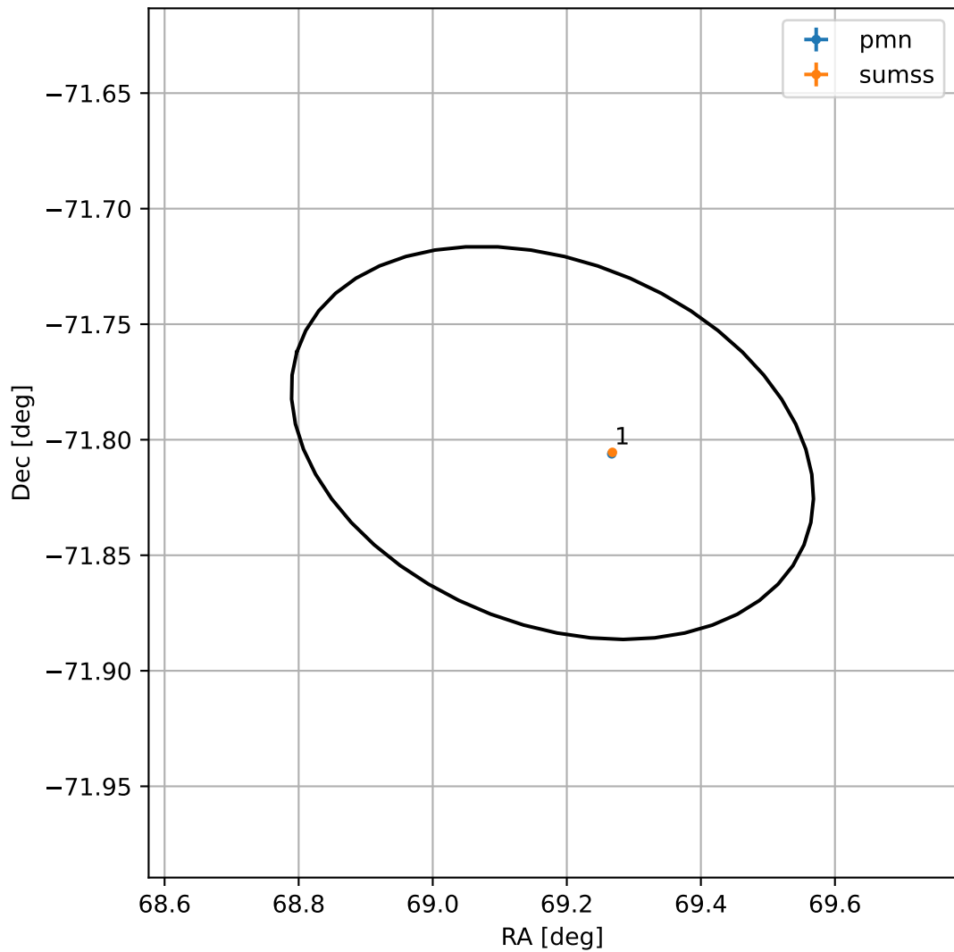
4FGL J0436.7-7148
