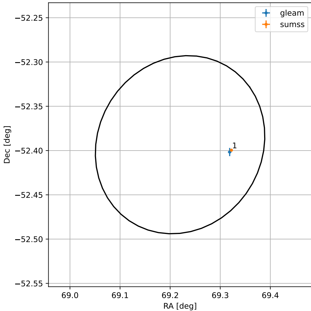
4FGL J0436.8-5223
