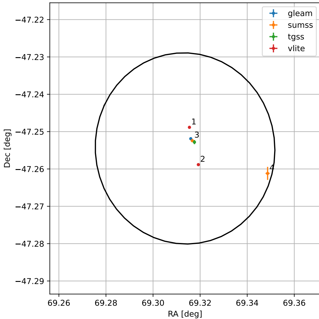
4FGL J0437.2-4715
