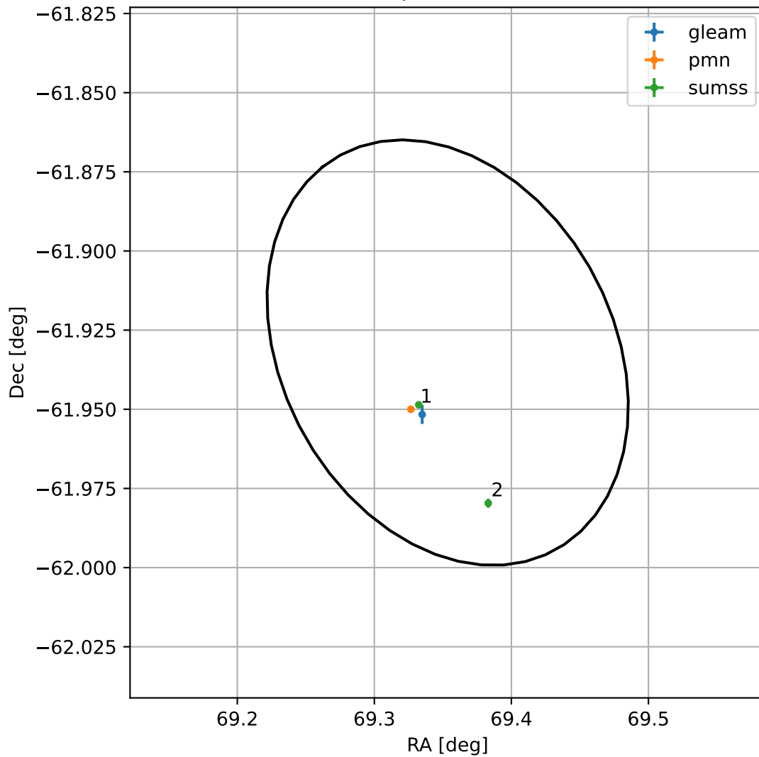
4FGL J0437.4-6155
