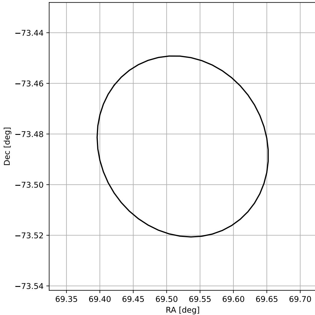
4FGL J0438.0-7329
