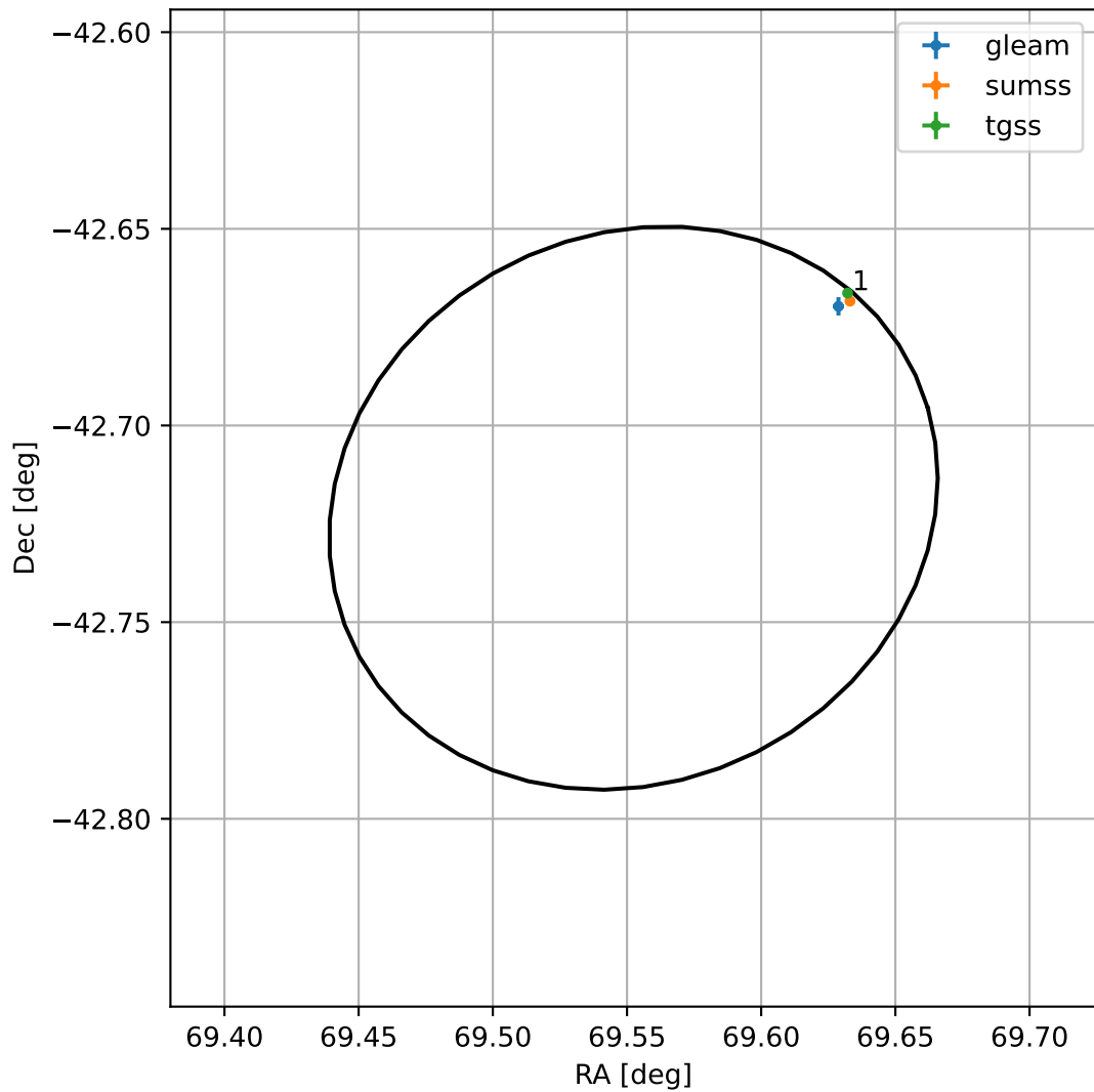
4FGL J0438.2-4243
