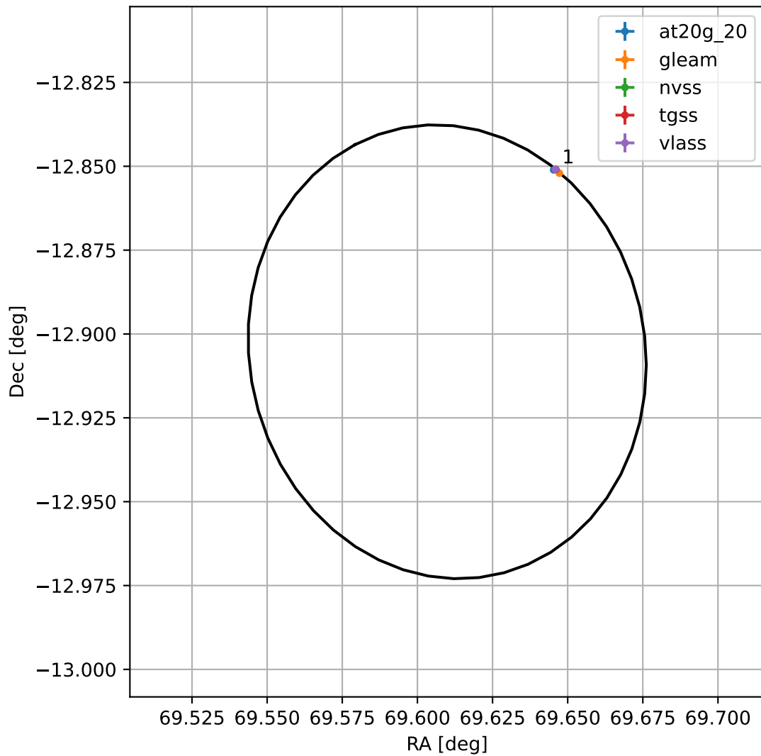
4FGL J0438.4-1254
