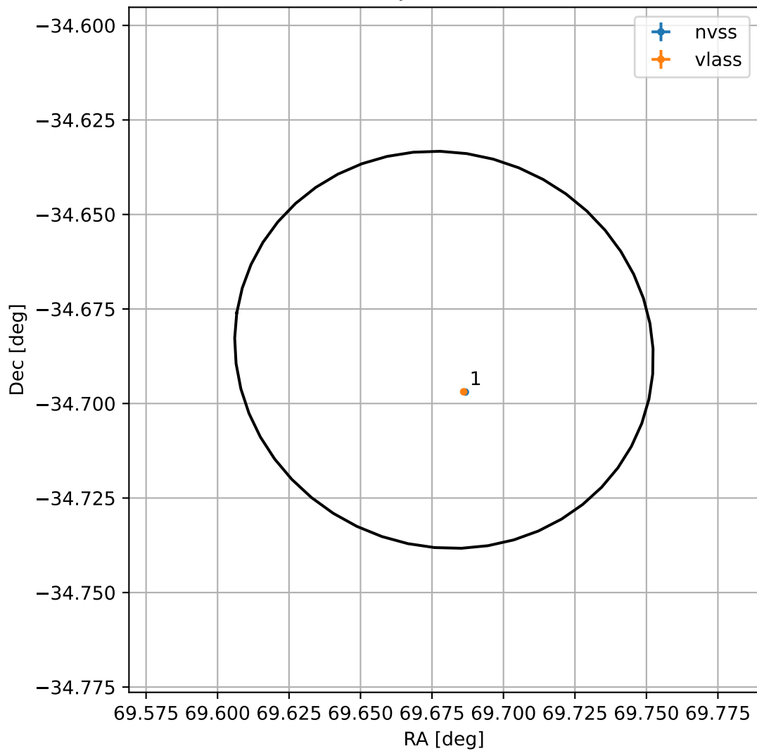
4FGL J0438.7-3441
