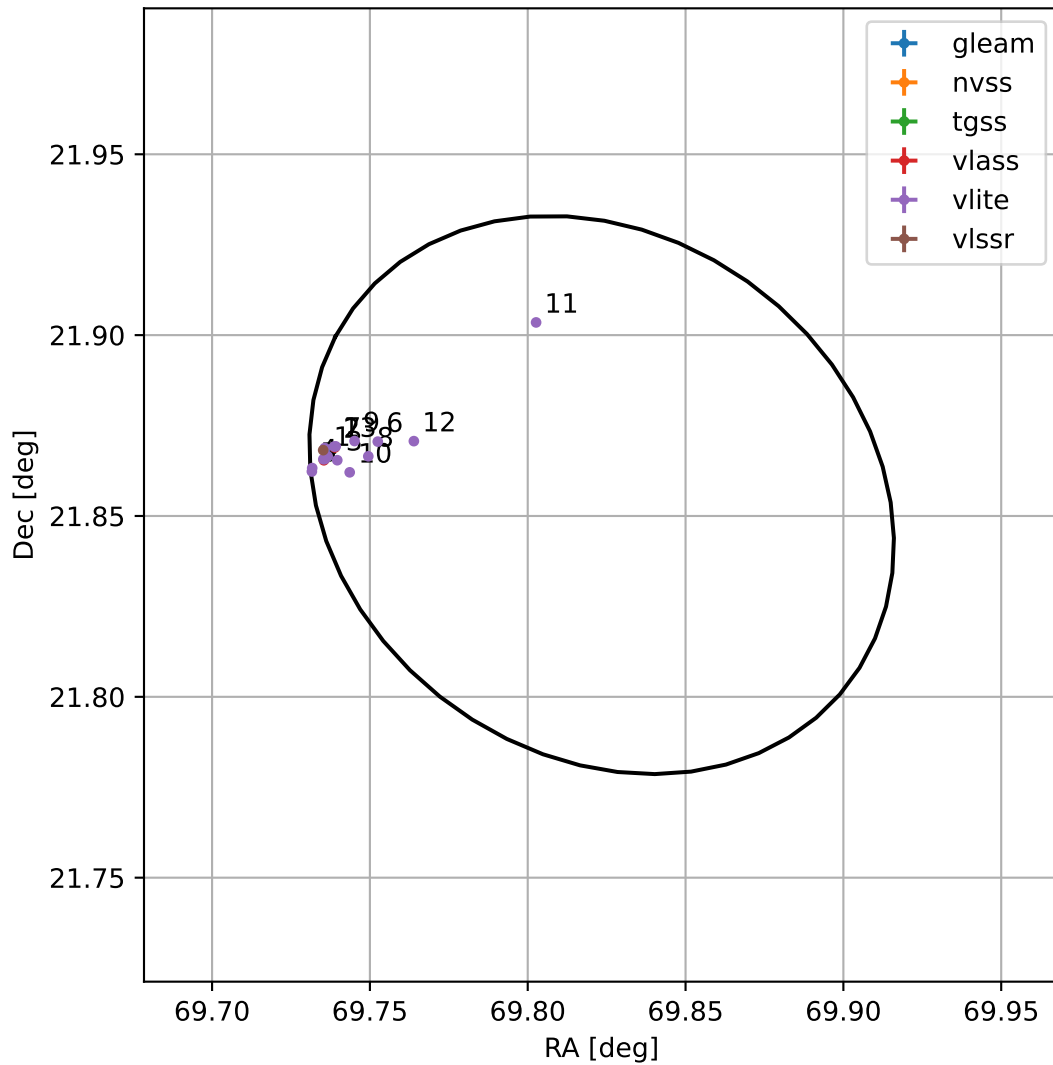
4FGL J0439.2+2151
