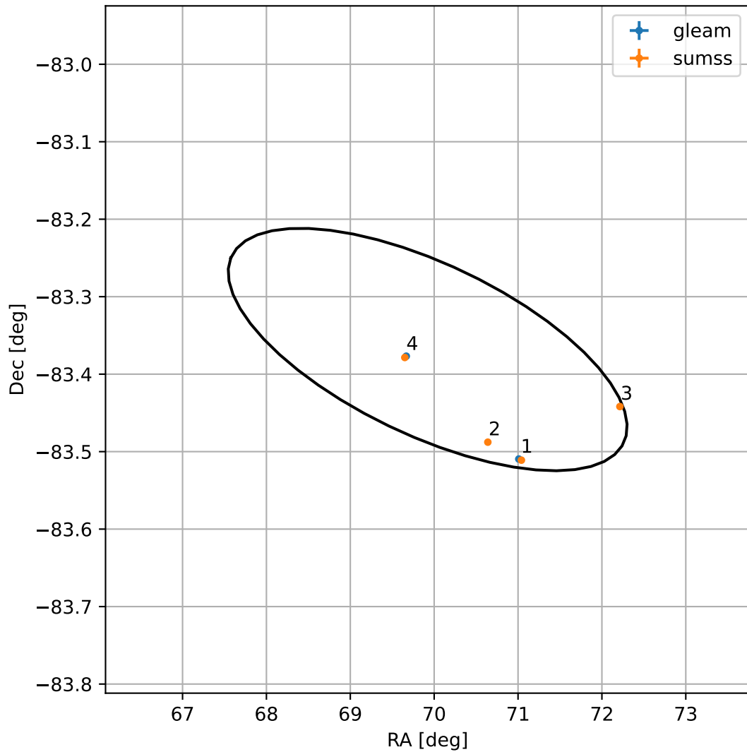
4FGL J0439.6-8322
