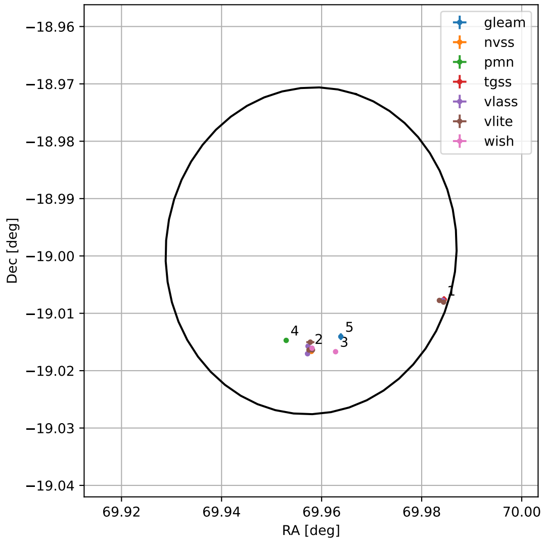
4FGL J0439.8-1859
