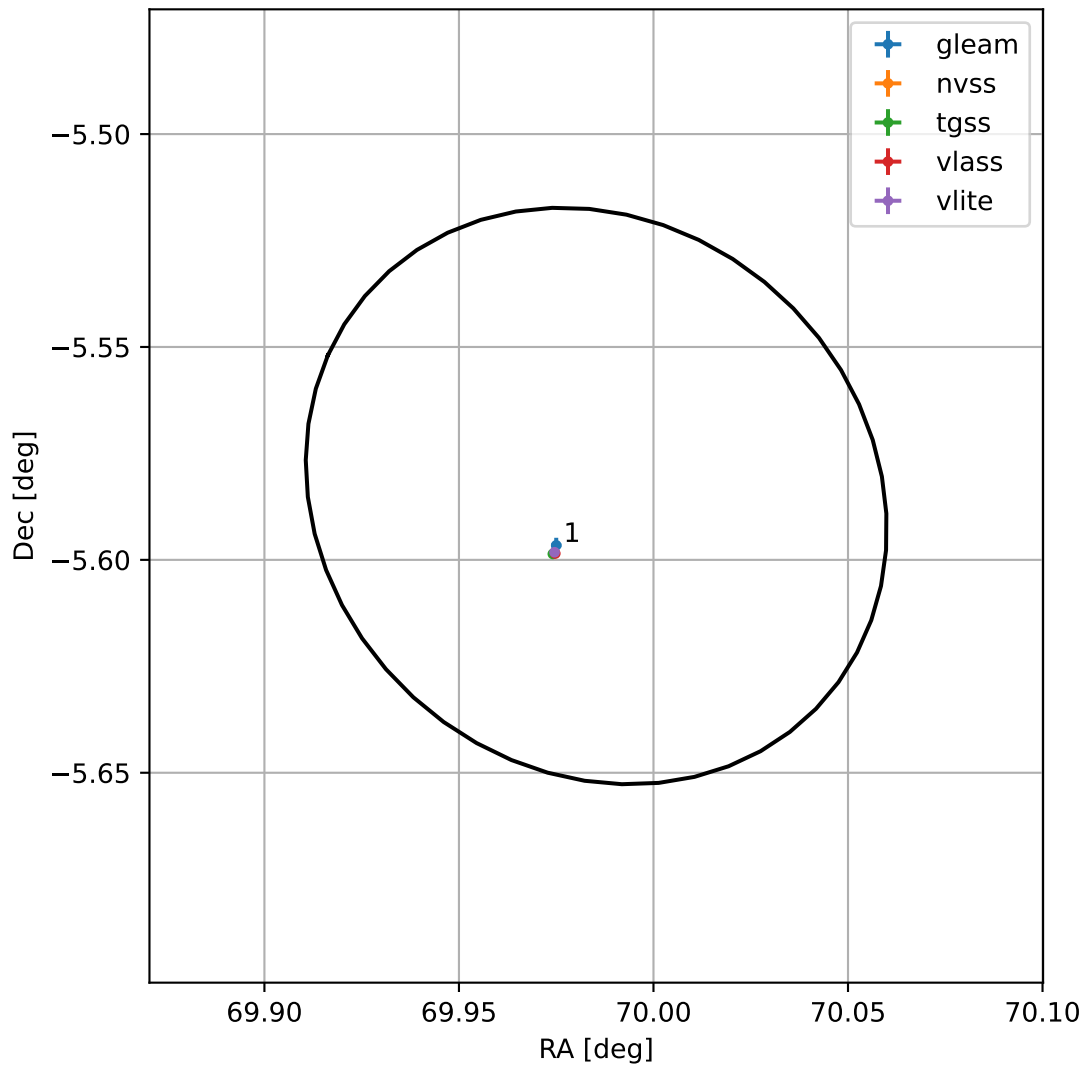
4FGL J0439.9-0535
