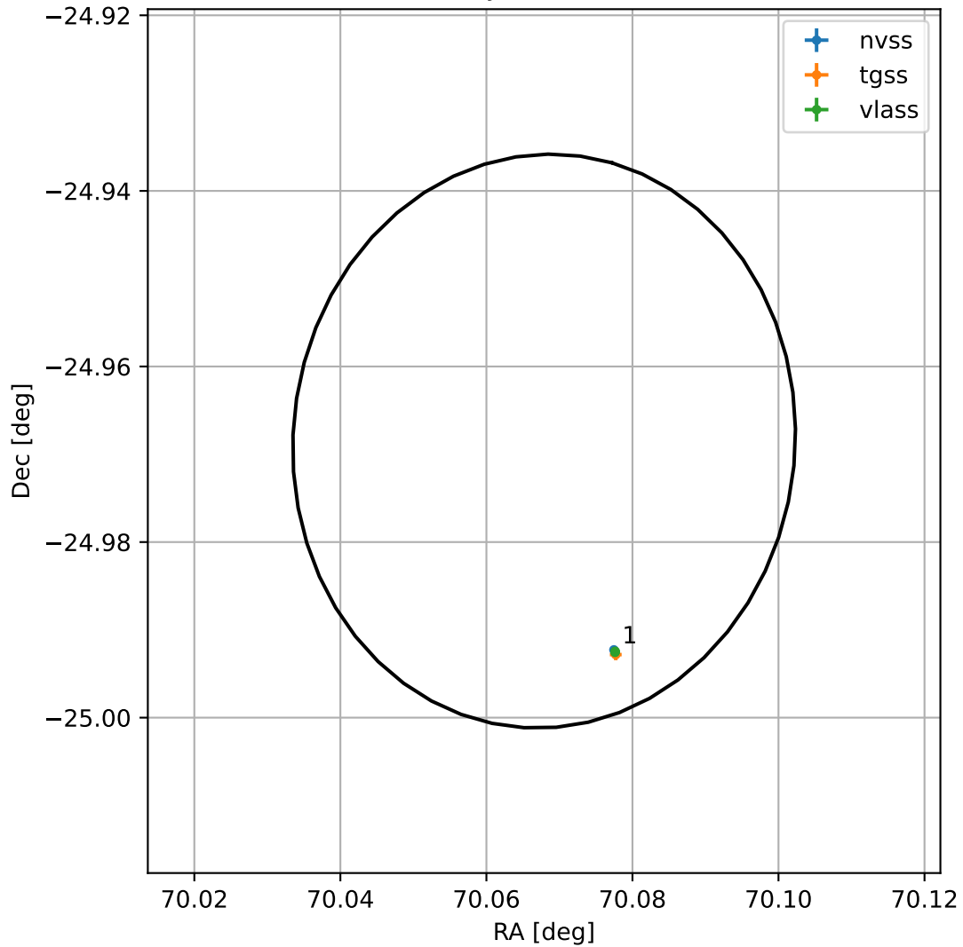
4FGL J0440.2-2458
