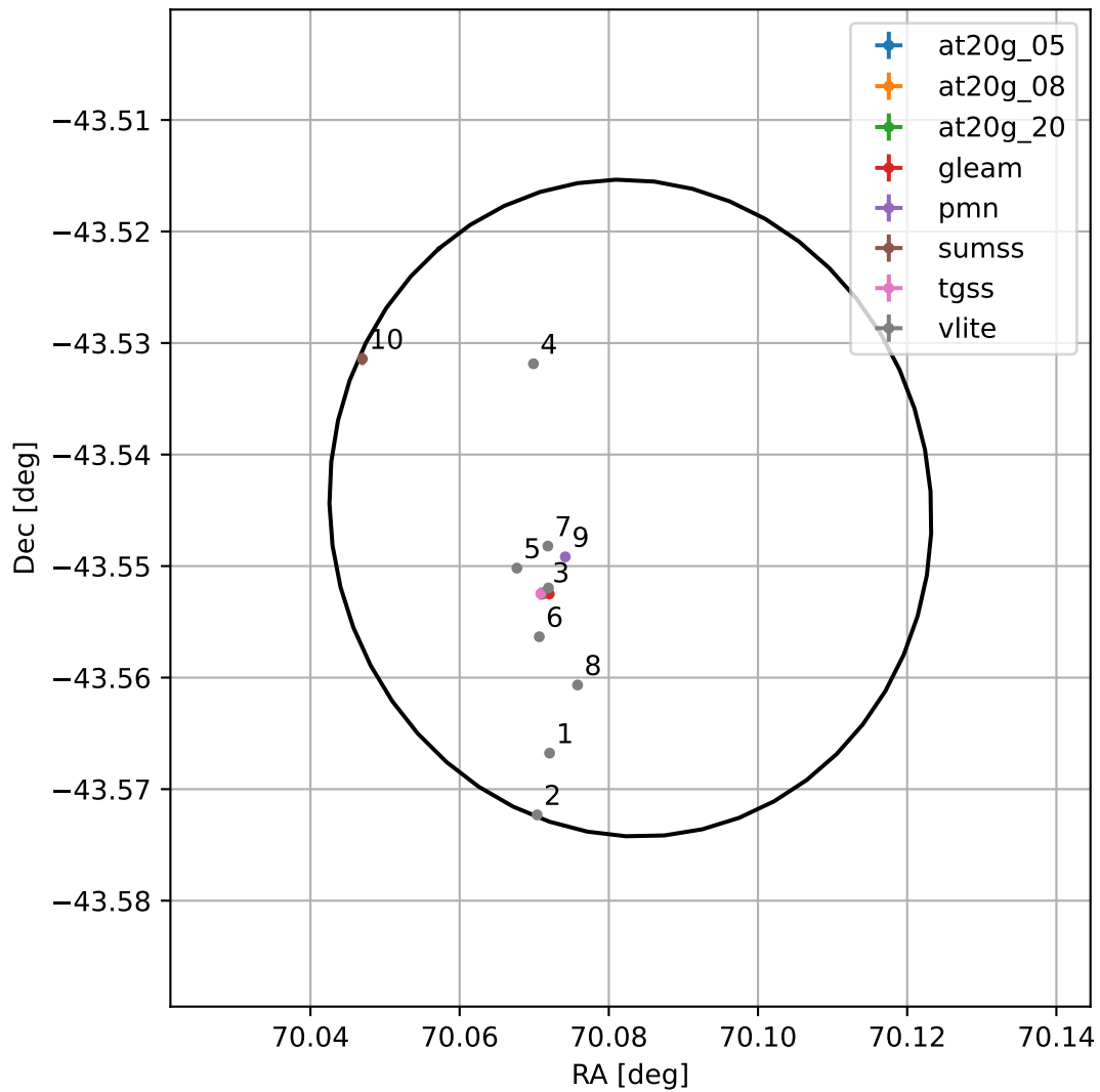
4FGL J0440.3-4332
