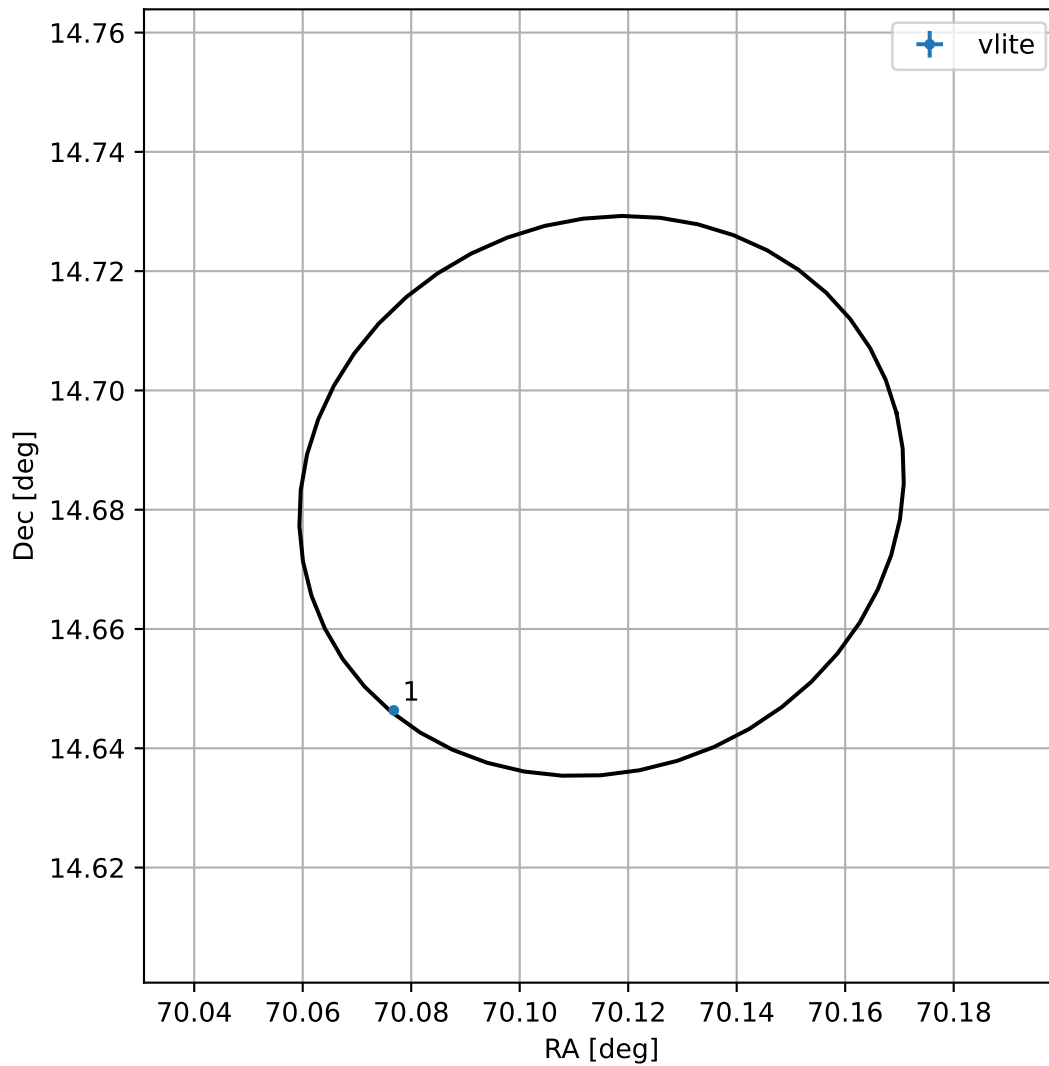
4FGL J0440.4+1440
