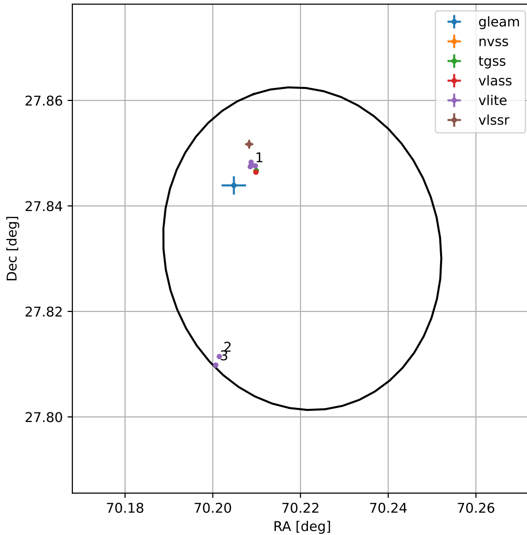
4FGL J0440.8+2749
