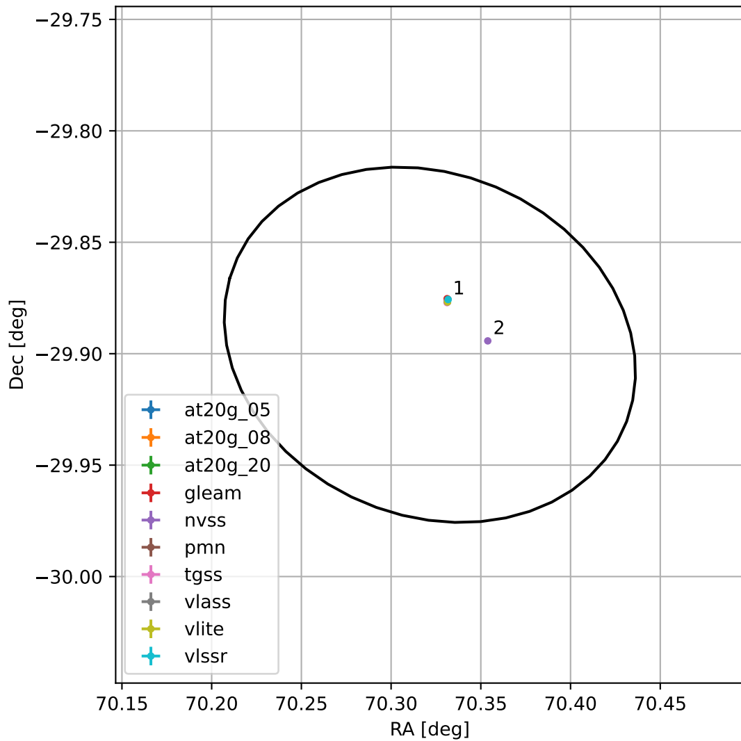
4FGL J0441.2-2953
