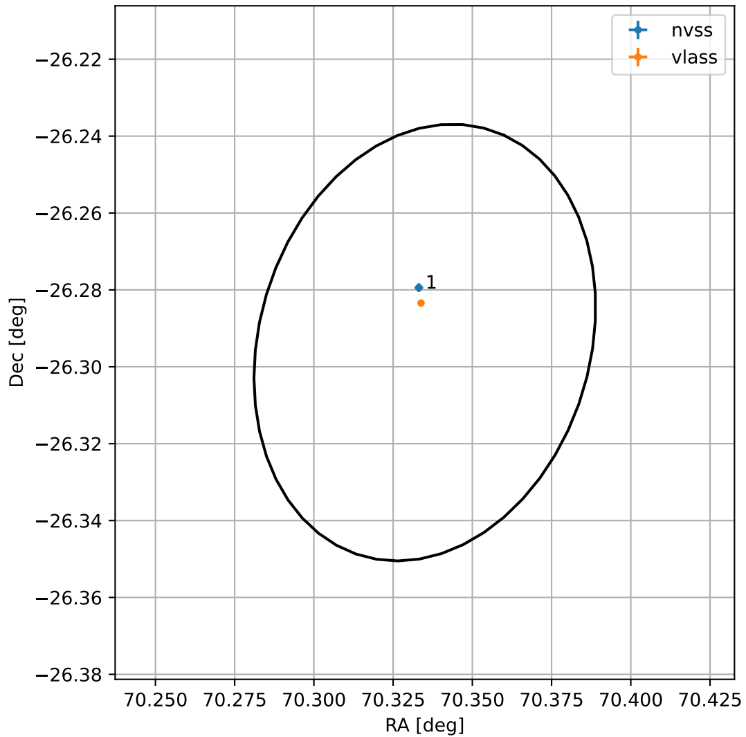
4FGL J0441.3-2617
