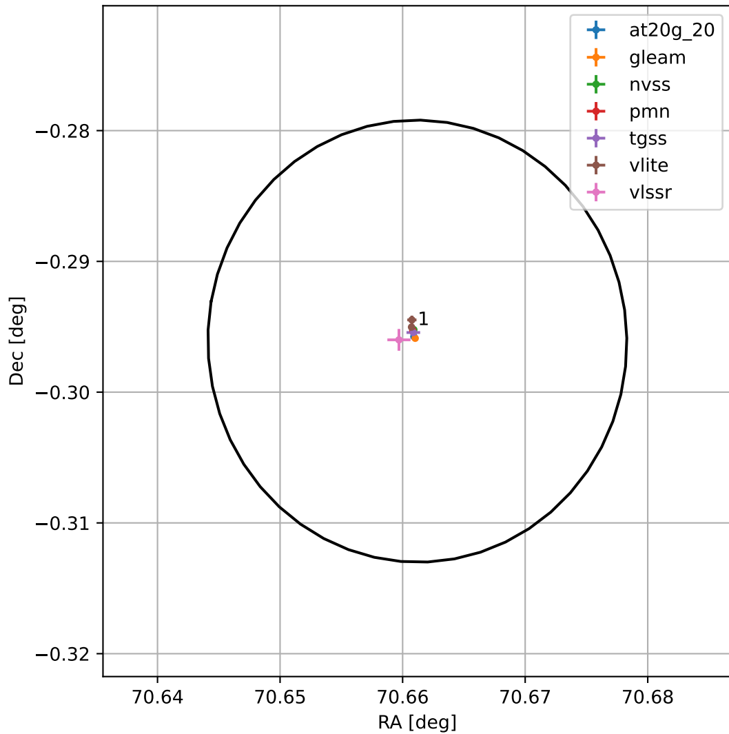
4FGL J0442.6-0017
