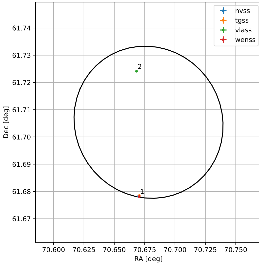
4FGL J0442.7+6142
