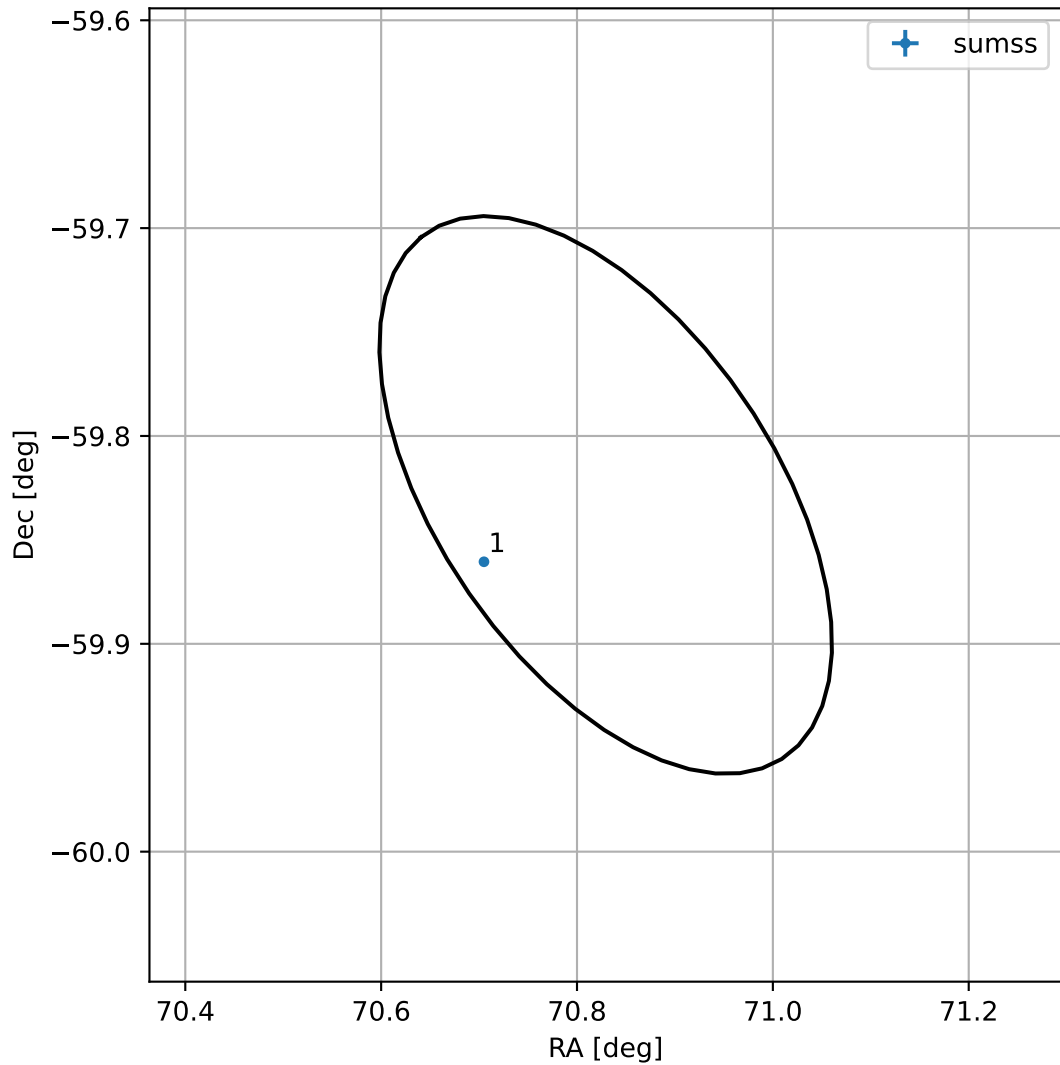
4FGL J0443.3-5949
