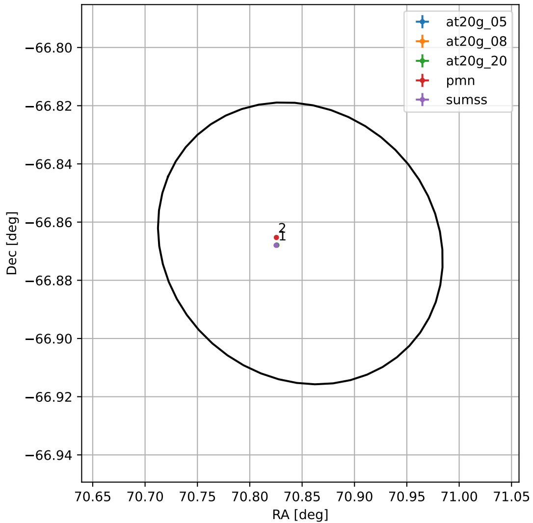
4FGL J0443.3-6652
