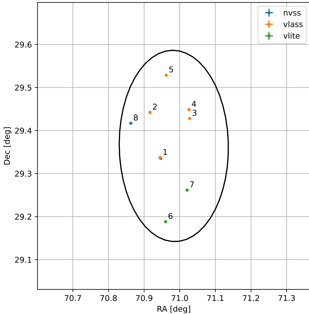
4FGL J0443.9+2921
