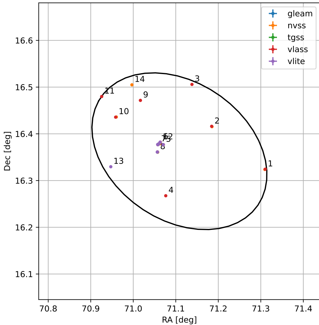
4FGL J0444.4+1621
