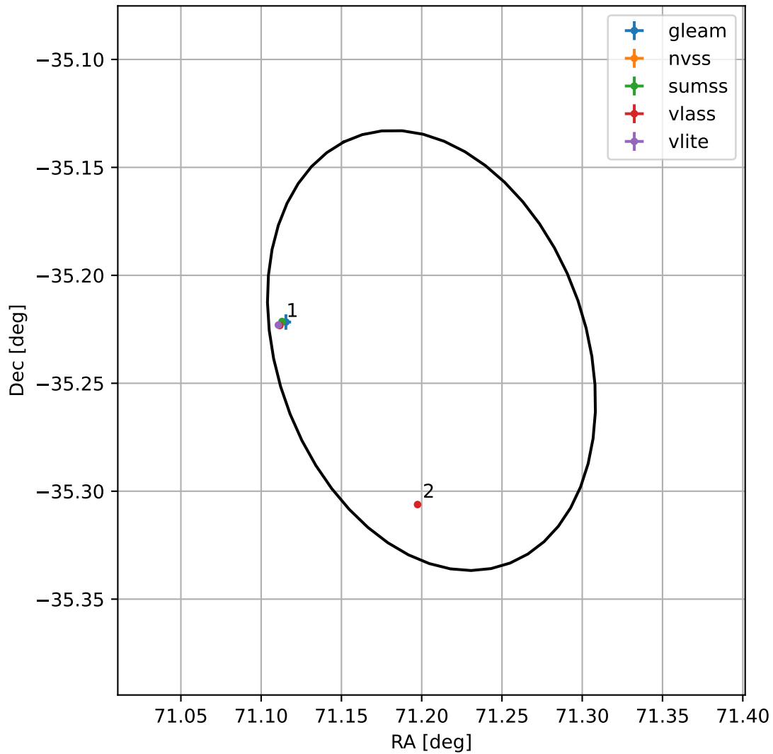
4FGL J0444.8-3514
