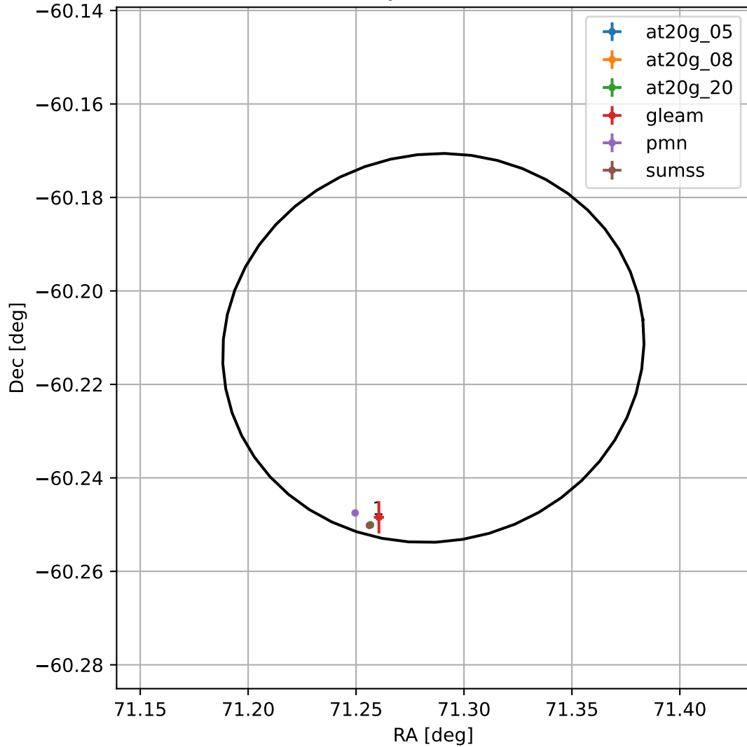
4FGL J0445.1-6012
