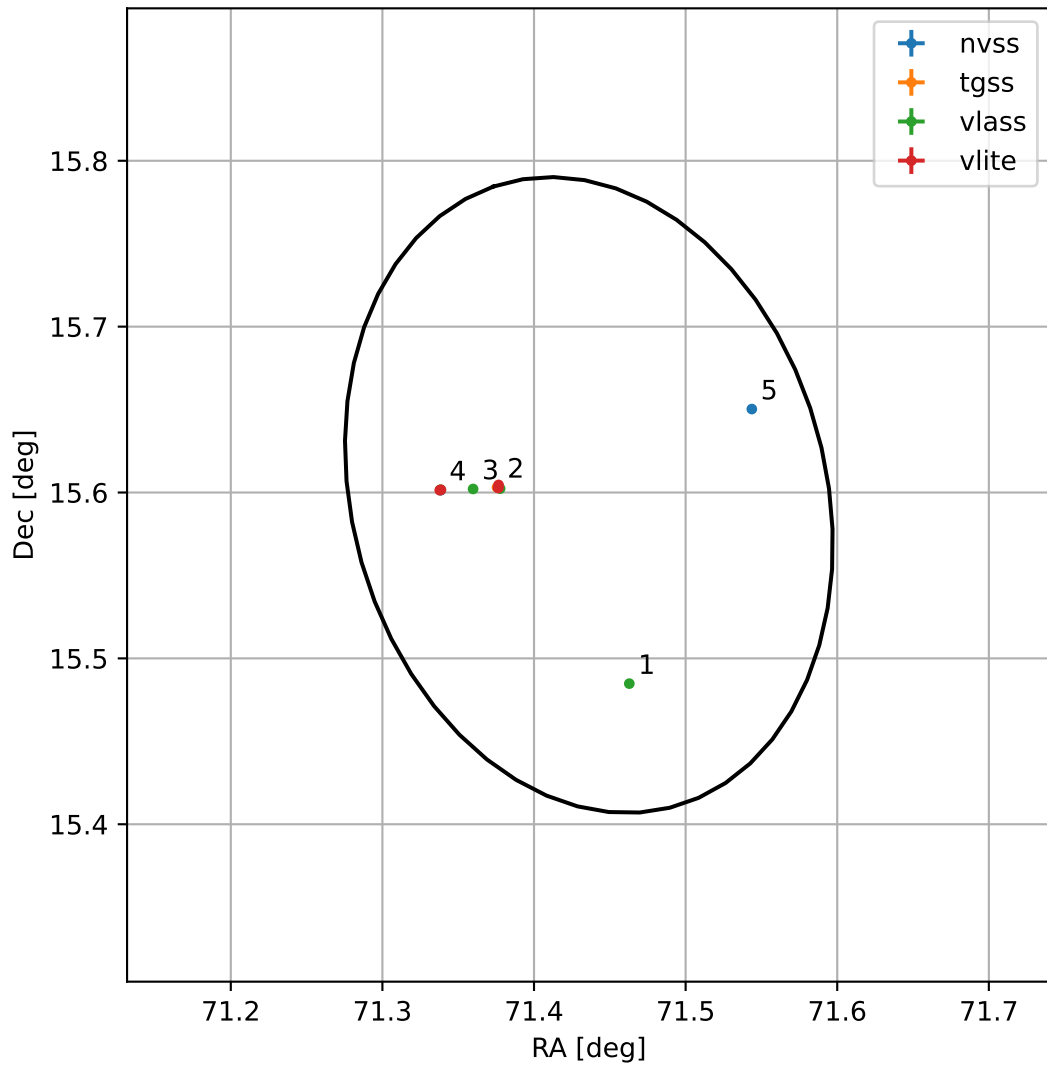
4FGL J0445.7+1535
