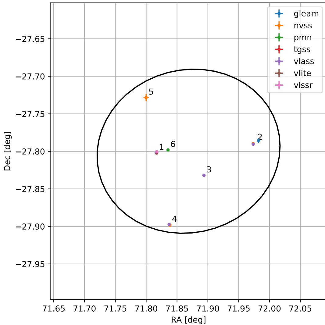
4FGL J0447.4-2747
