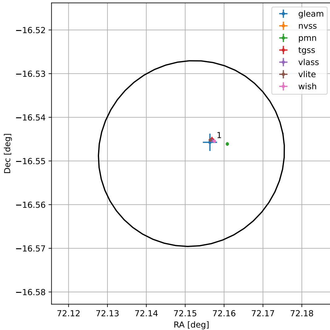
4FGL J0448.6-1632
