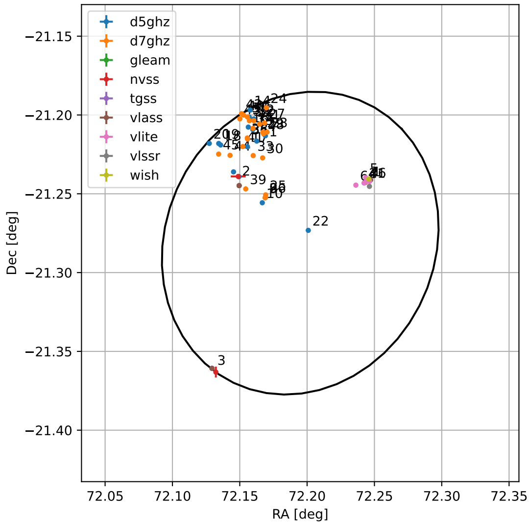
4FGL J0448.7-2116
