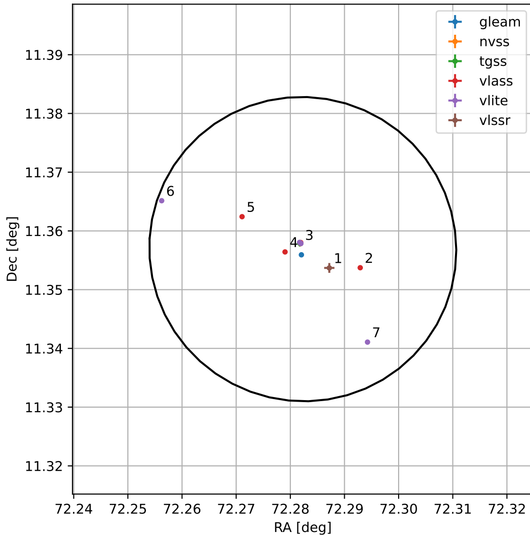
4FGL J0449.1+1121
