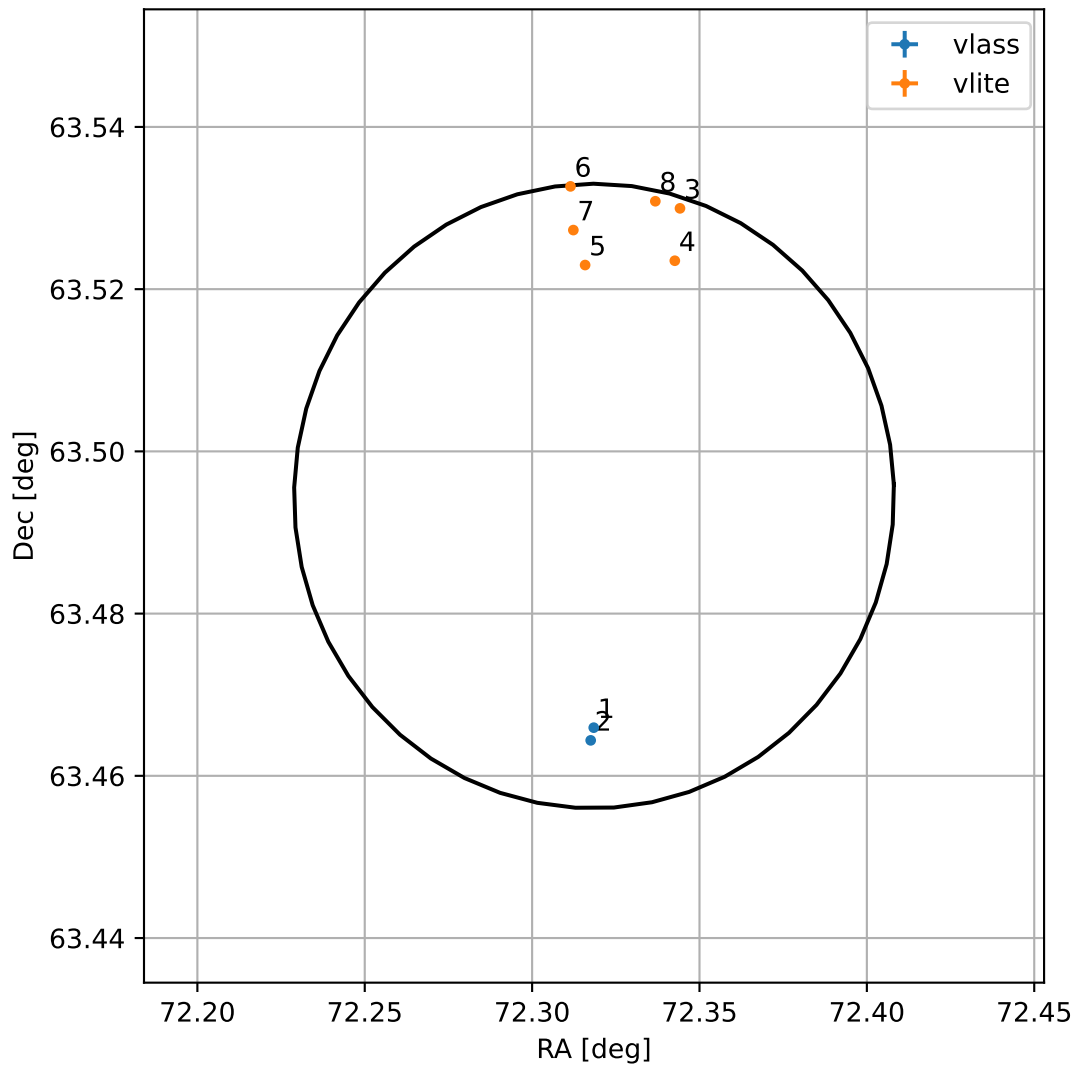
4FGL J0449.2+6329
