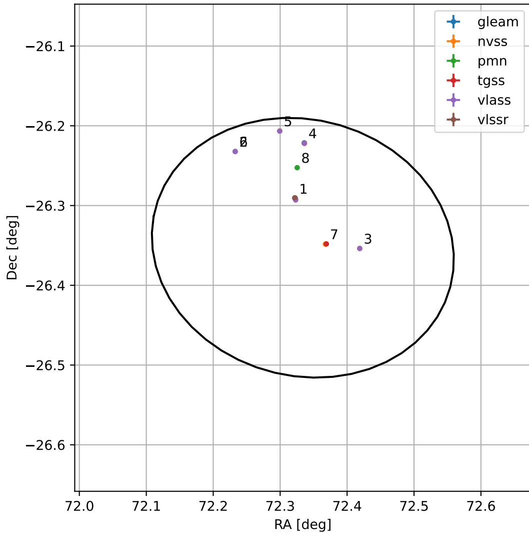
4FGL J0449.3-2621
