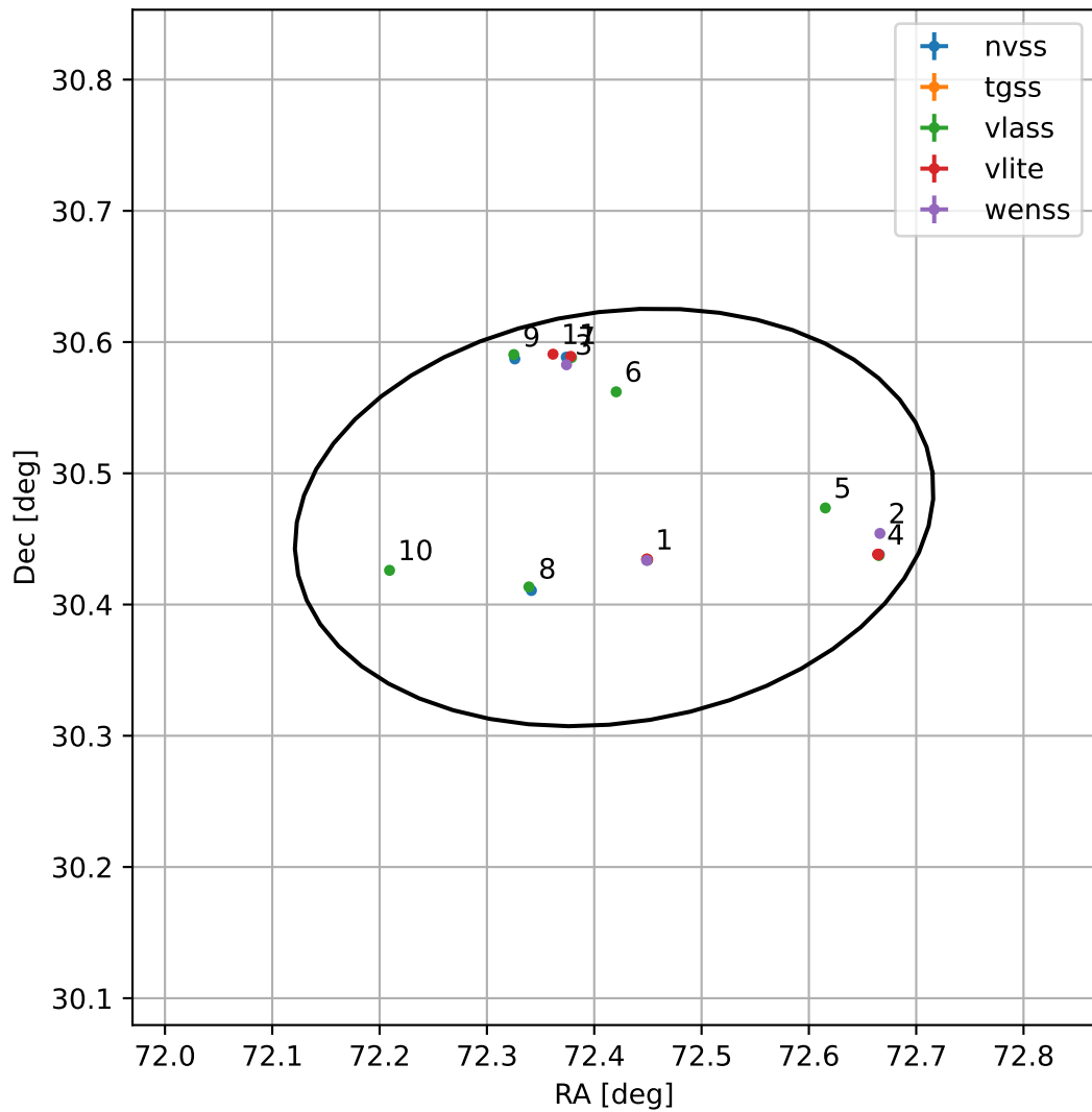
4FGL J0449.6+3027
