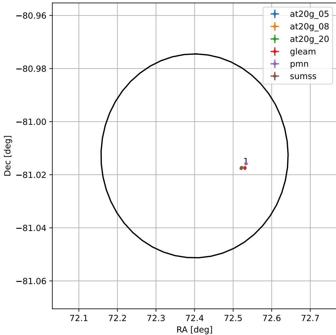
4FGL J0449.6-8100
