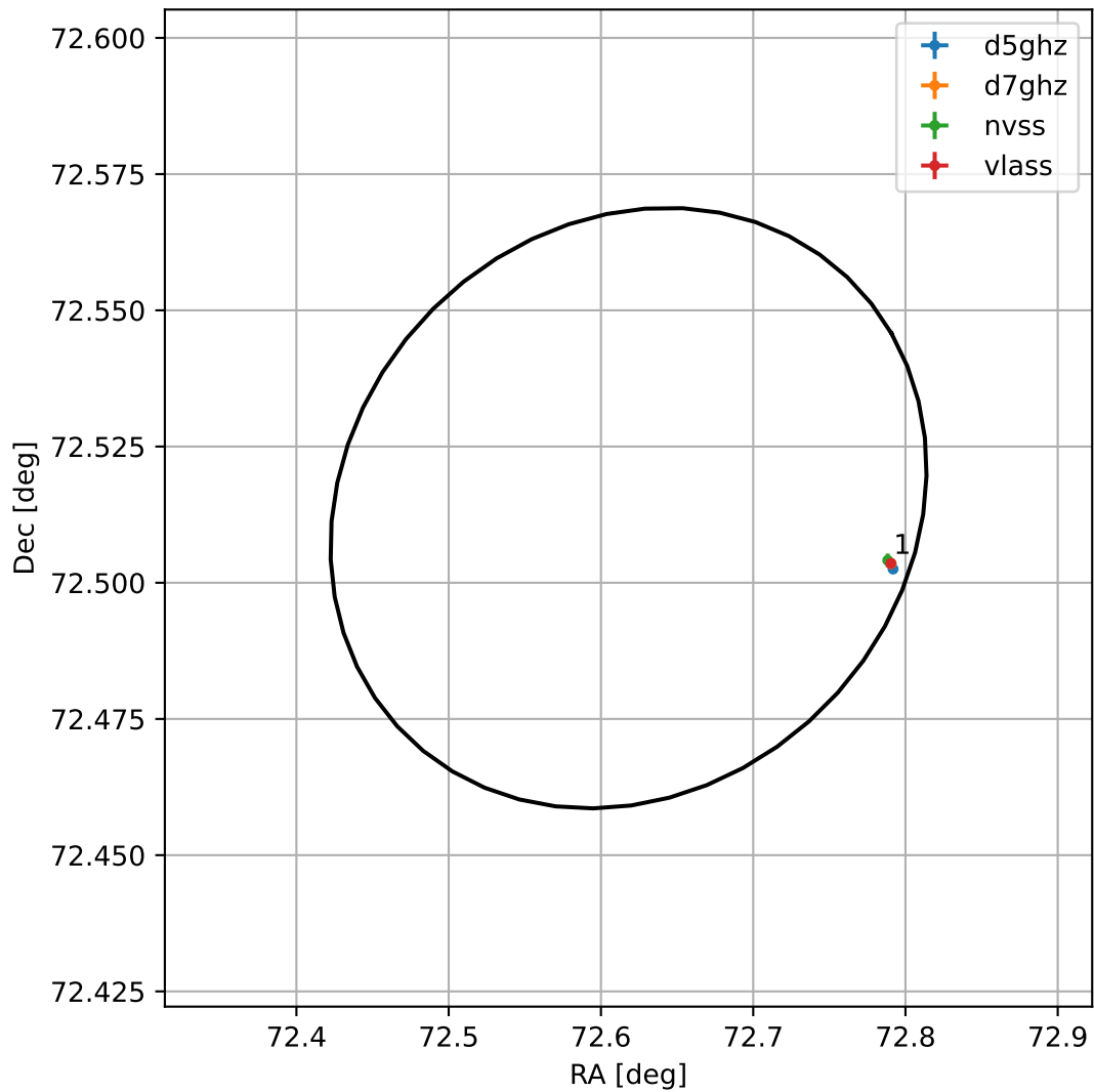
4FGL J0450.4+7230
