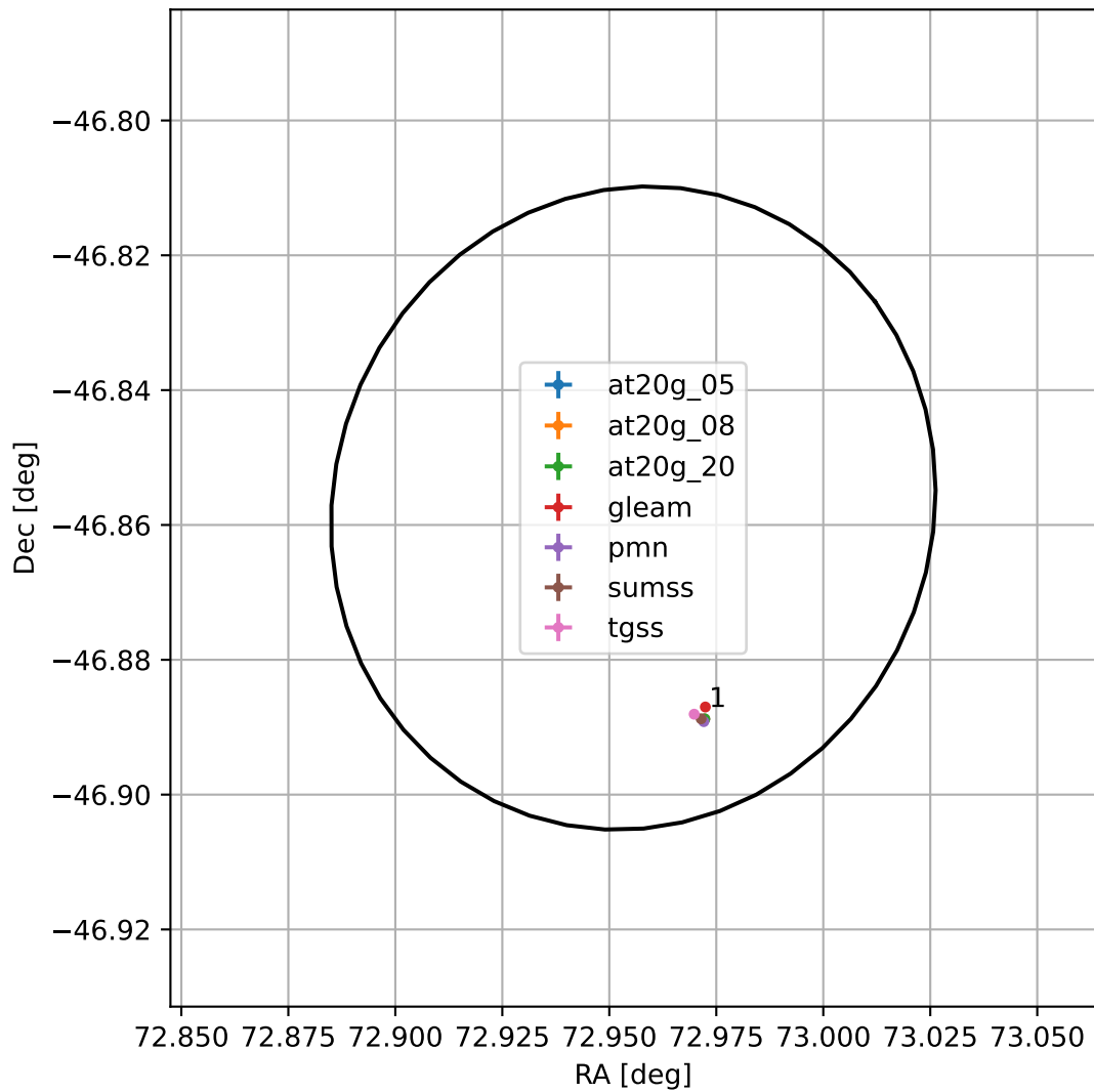
4FGL J0451.8-4651
