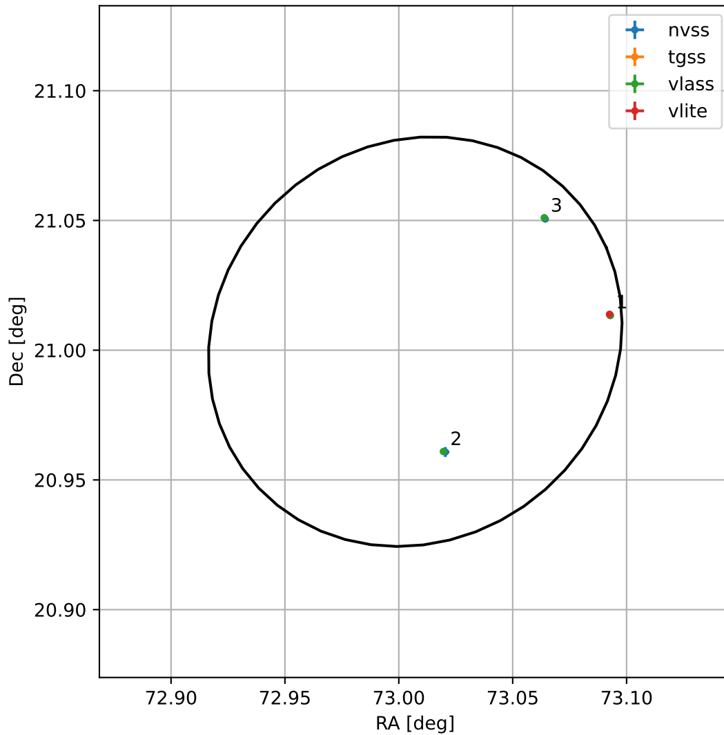
4FGL J0452.0+2100
