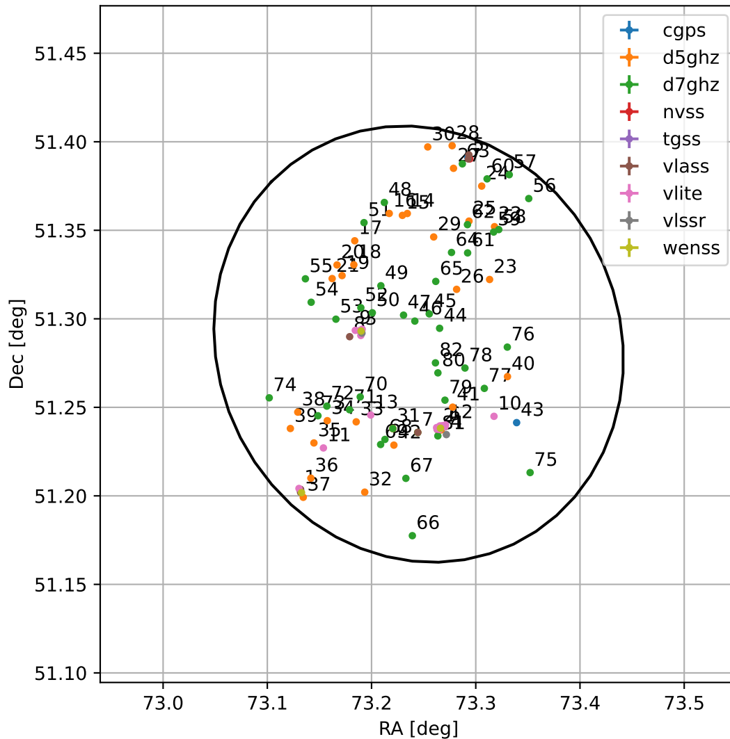
4FGL J0452.9+5117
