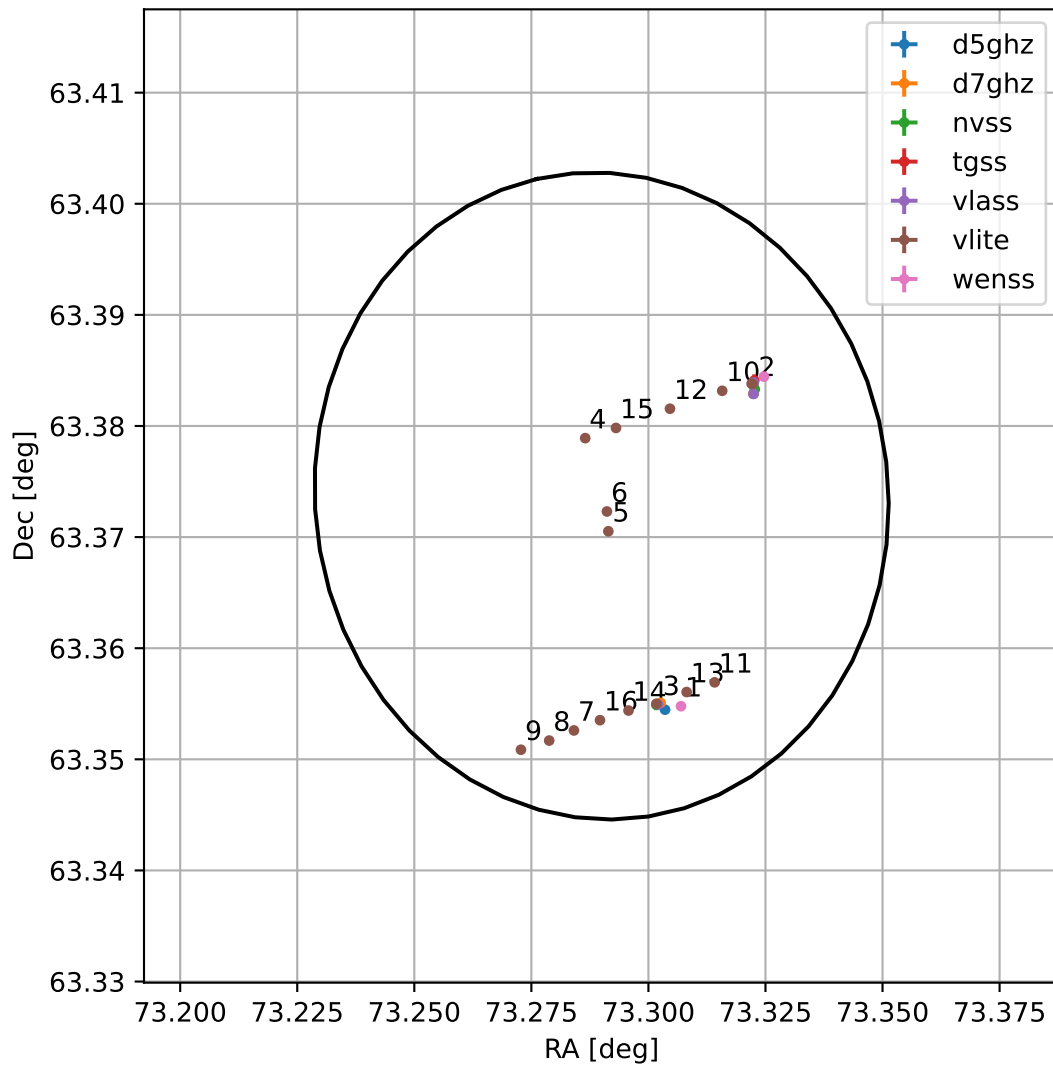
4FGL J0453.1+6322
