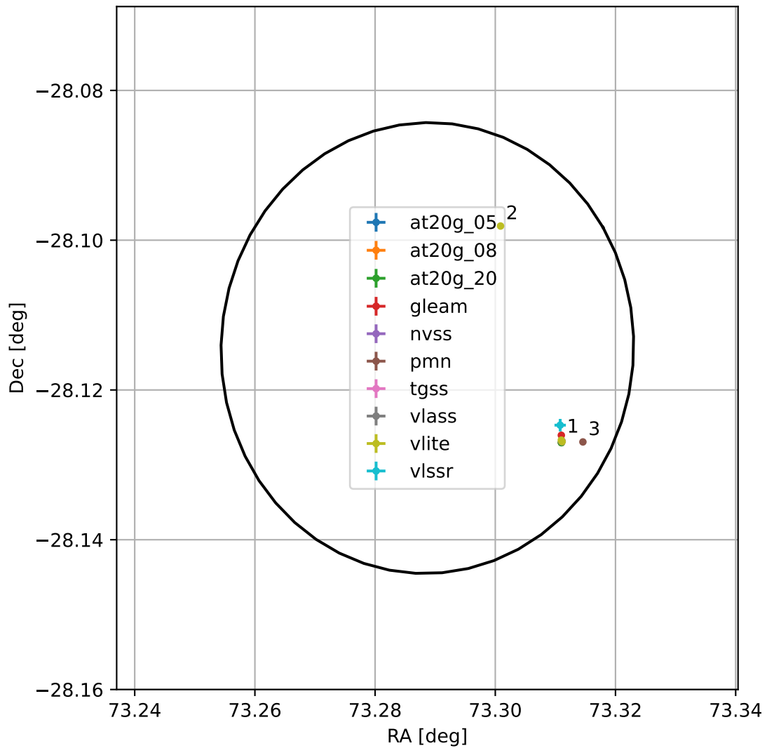
4FGL J0453.1-2806
