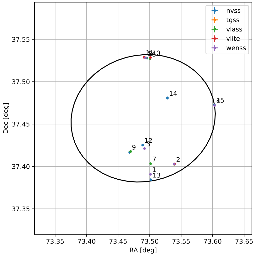
4FGL J0453.9+3727
