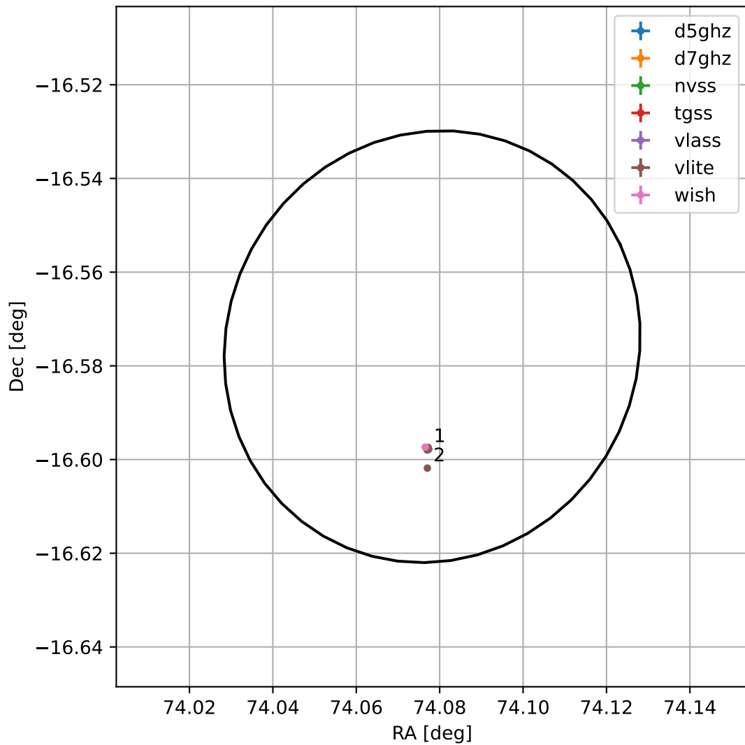
4FGL J0456.3-1634
