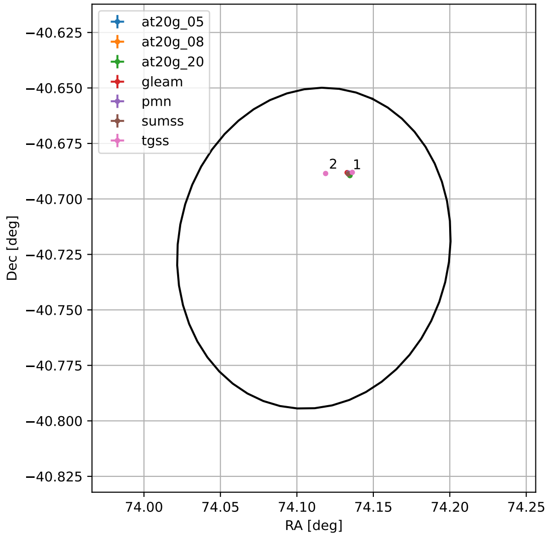
4FGL J0456.4-4043
