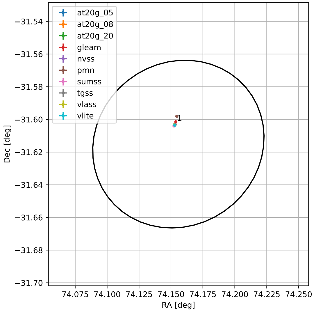
4FGL J0456.6-3136
