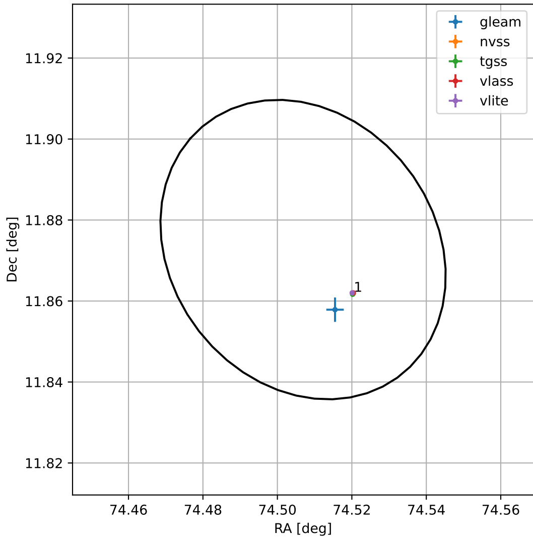
4FGL J0458.0+1152
